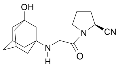
Vildagliptin
